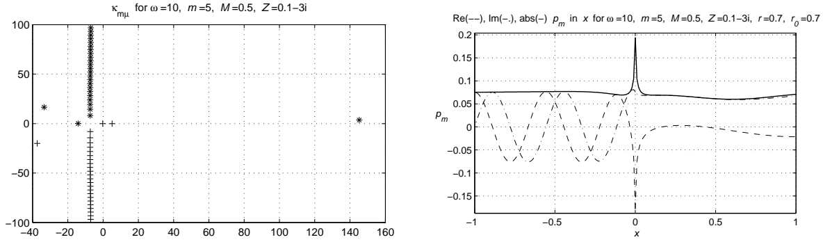
Figure 7.11 Eigenvalues \kappa_{m\mu}^{\pm} and \text{Re}(p_m) , \text{Im}(p_m) and |p_m| is plotted of the m = 5 -th component of the point source field in a lined flow duct with \omega = 10 , Z = 0.1 - 3i , x_0 = 0 , r_0 = 0.7 , M = 0.5 at r = 0.7 and \theta = \theta_0 . Note the presence of 3 surface waves.
